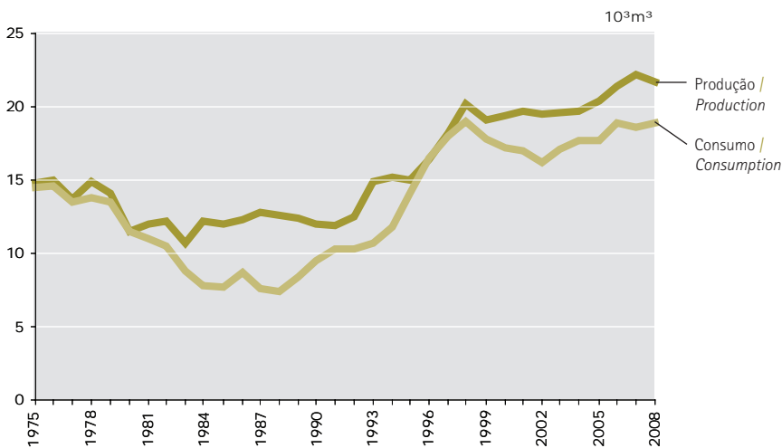
Chart 2.8 | Gasoline
