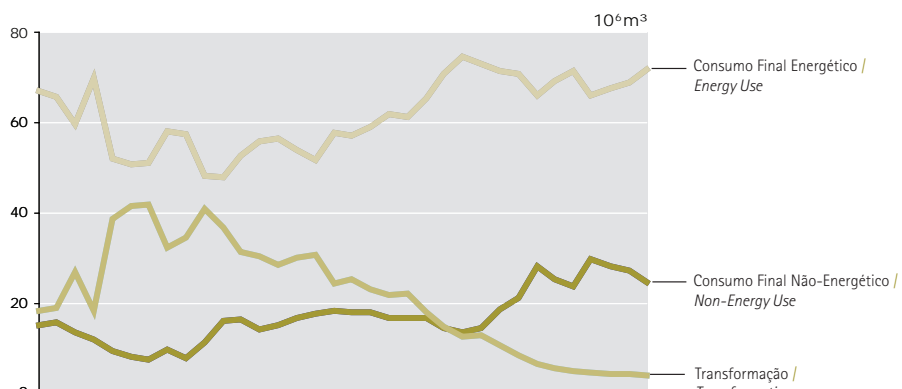
Chart 2.3 | Natural Gas
