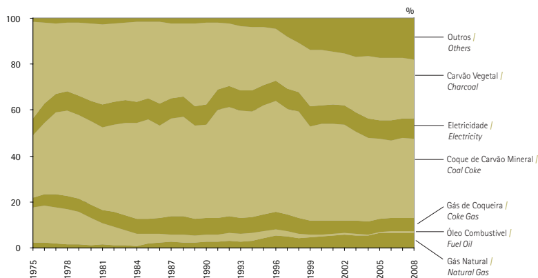
Chart 3.7 | Pig-Iron and Steel Sector Energy Consumption
